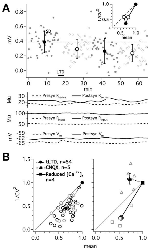
Figure 2. CV Analysis of tLTD Indicates a Presynaptic Expression Mechanism
